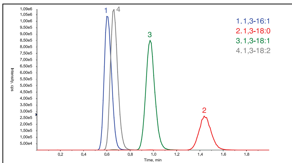
Deuterated DG Mixture II Avanti Number LM-6004
