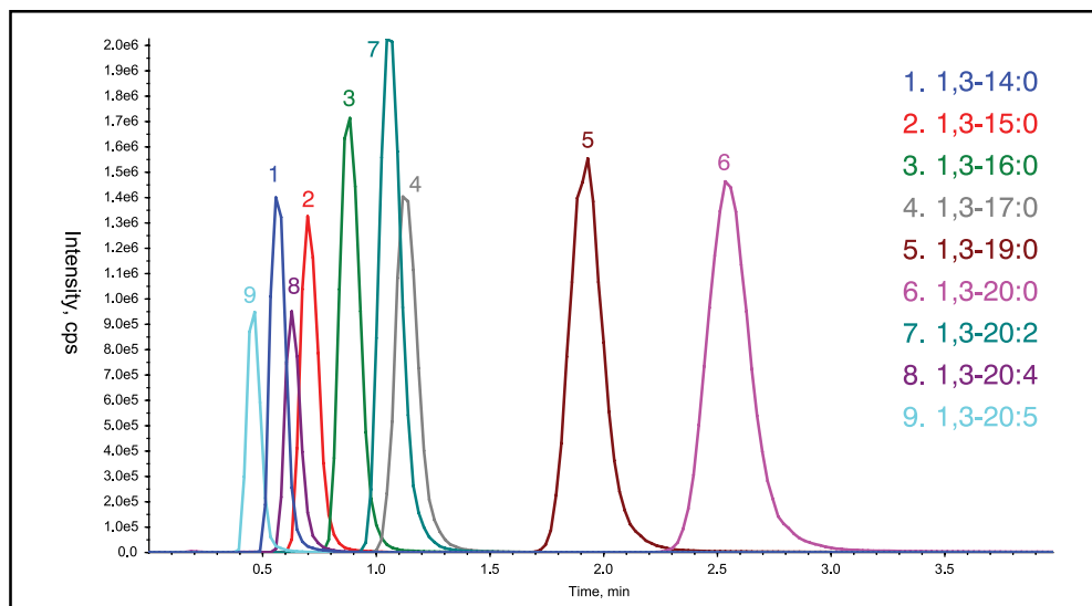
Deuterated DG Mixture I Avanti Number LM-6001
