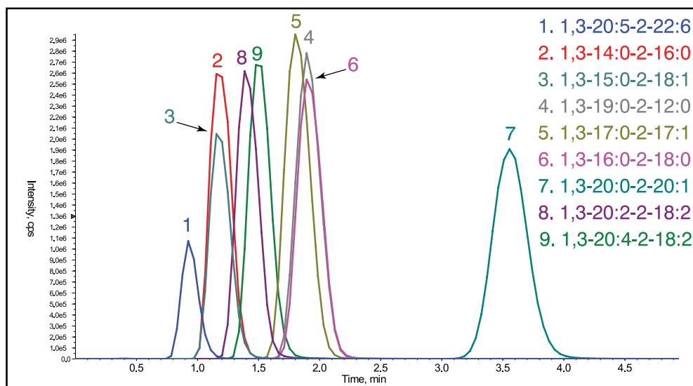
Deuterated TG Mixture I Avanti Number LM-6000
