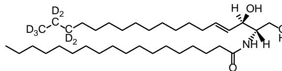
C18 Ceramide-d7 (d18:1-d7/18:0)
