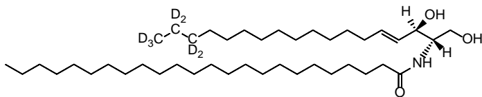
C24 Ceramide-d7 (d18:1-d7/24:0)
